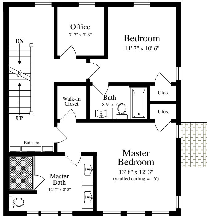
SECOND FLOOR (ceiling = 8' 3")
