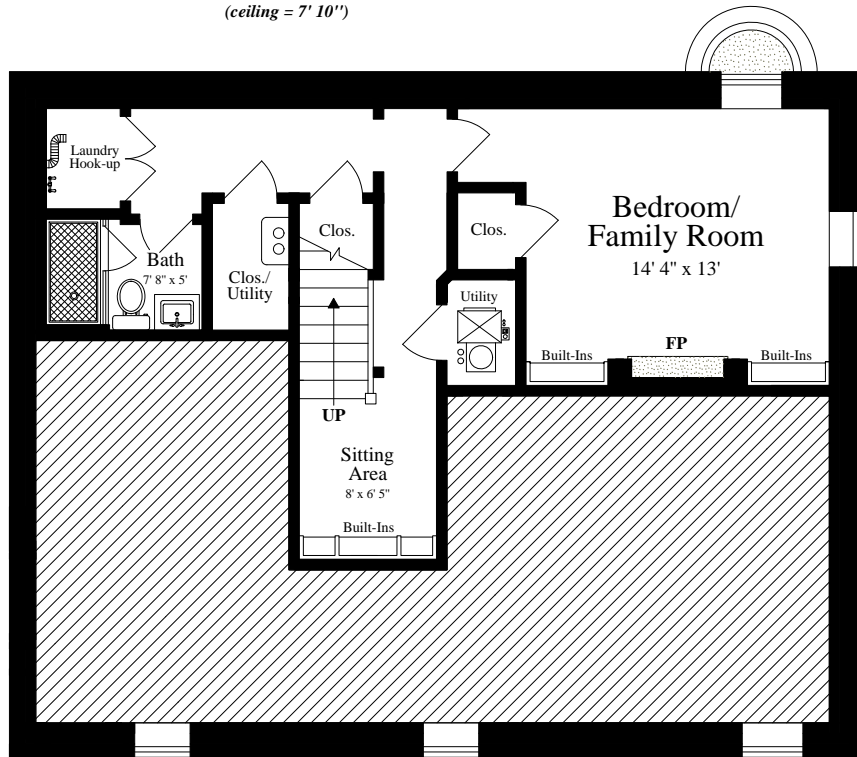
LOWER LEVEL (ceiling = 7' 2")
