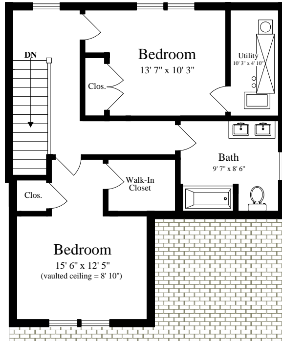
THIRD FLOOR (ceiling = 7' 10")
